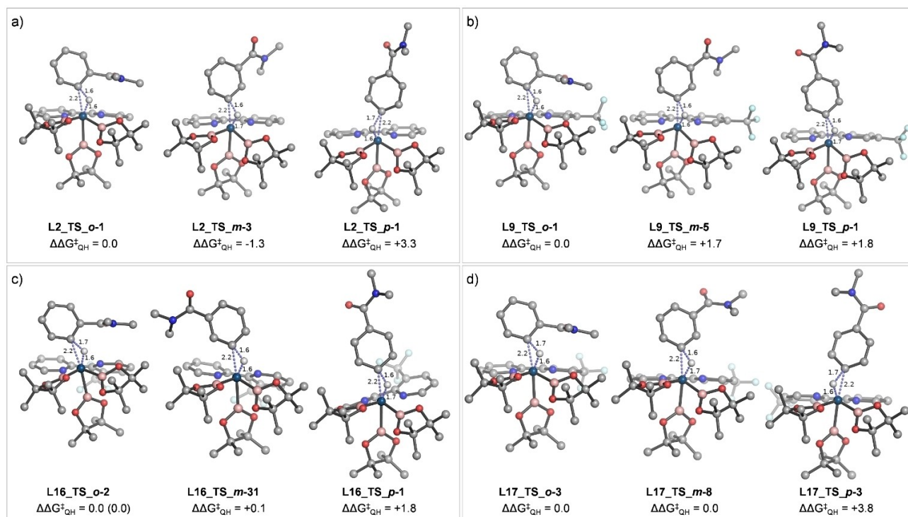
Figure 4. Low energy outer-sphere transition states (TS) calculated for the oxidative addition step between N,N -dimethylbenzamide ( 1a ) and Ir III (ligand)(Bpin) 3 (ligand = L2 (a), L9 (b), L16 (c) and L17 (d); o = ortho , m = meta , p = para ). Relative activation free energies ( \Delta\Delta G^{\ddagger}_{\text{QH}} ) calculated with SMD THF /M06/6-311G(2d,p) + SDD(Ir)//M06/6-31G(d) + LANL2DZ(Ir) are given in kcal mol -1 . Metal-ligand and breaking/forming C–H, Ir–C and Ir–H bonds are represented as blue dashed lines, respectively. Non-reactive hydrogens have been omitted for clarity.
