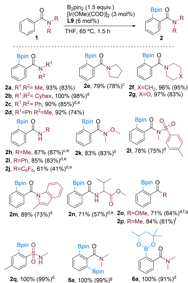
Scheme 1. Borylation of benzamides and related precursors. Reaction conditions: substrate (0.25 mmol), B 2 pin 2 (0.375 mmol, 1.5 equiv), [Ir(OMe)(COD)] 2 (3 mol%), L9 (6 mol%), THF (0.2 M), 65 °C, 1.5 h. 1 H NMR yield using CH 2 Br 2 as IS (mean value of 3 parallel reactions), isolated yield described between parenthesis [a] Reaction time 1 h. [b] Reaction time 2 h. [c] Reaction time 4 h. [d] Reaction time 24 h. [e] Reaction temperature 80 °C. [f] Reaction temperature 100 °C. [g] Ligand L14 was used. Note: only traces of diborylated products were detected.
